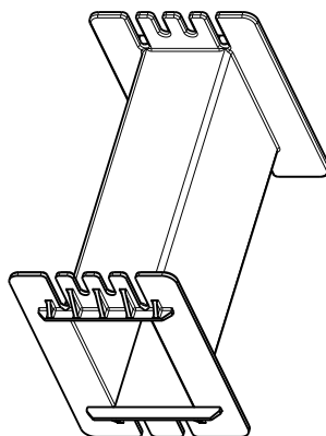
C-125 Bobbin
